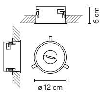
Built-in Canopy E3 Ø 120 mm.
